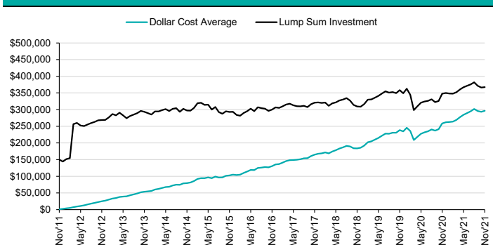
Figure 13 - Portfolio values
