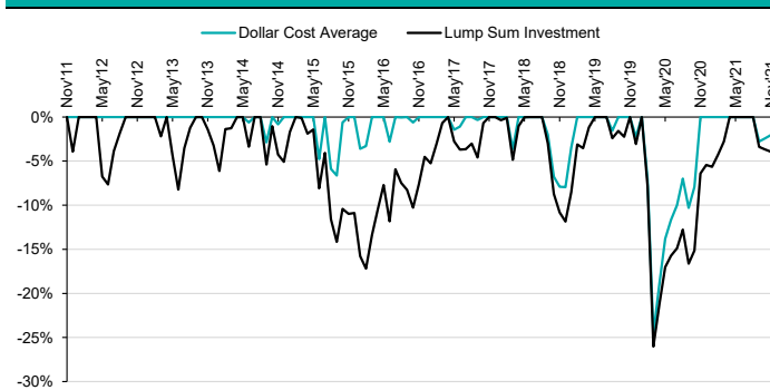
Figure 9 - Drawdowns
