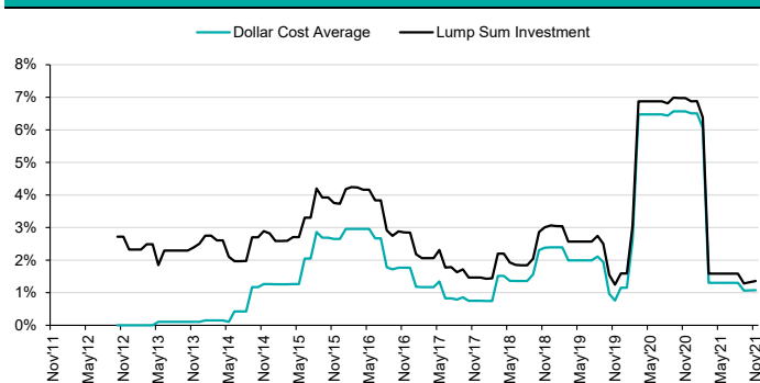
Figure 10 - Downside deviations
