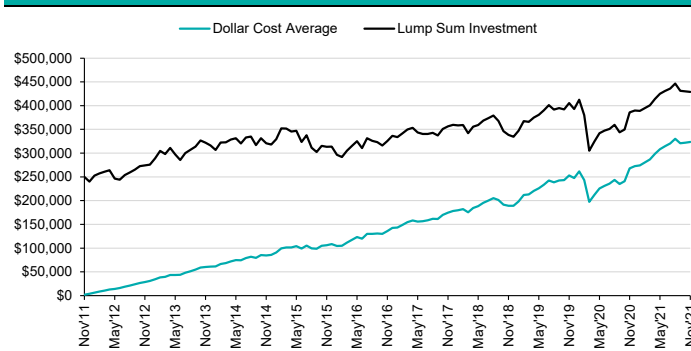
Figure 8 - Portfolio values
