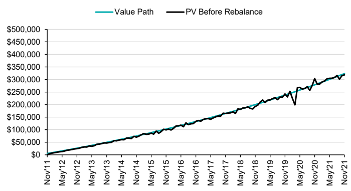
Figure 17 - Portfolio Value
