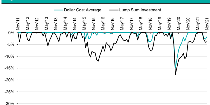
Figure 14 - Drawdowns
