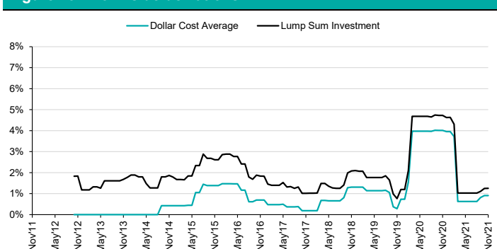
Figure 15 - Downside deviations
